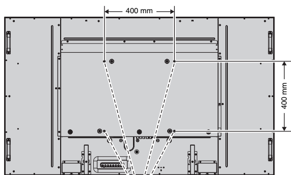
VESA Mounting Interface
