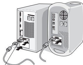
Macintosh Cable Adapter (not included) Note: Some Macintosh systems do not require a Macintosh Cable Adapter
