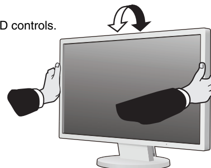
Figure TS.1
