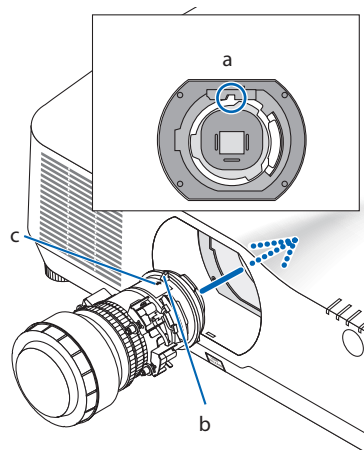
a: Guiding notch / b: Protrusion / c: Arrow
