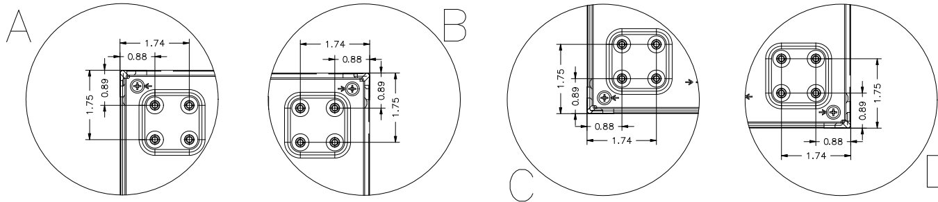
OPTIONAL MOUNTING HOLES M4 Depth 8mm FOR MOUNT UNIT
