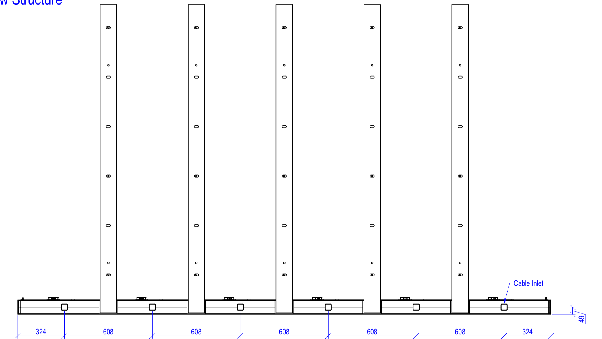
Rear View Structure
