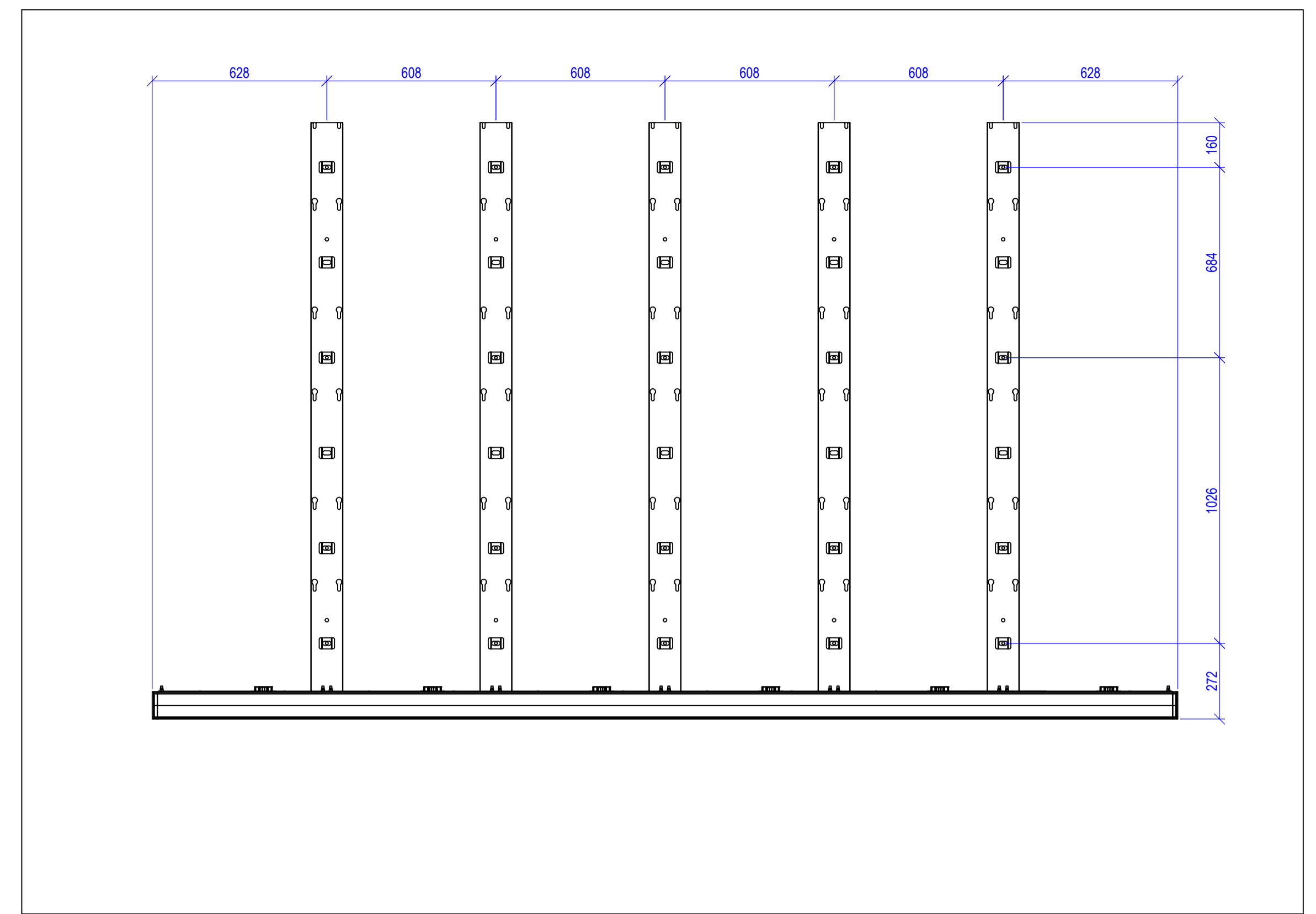
Front View Structure
