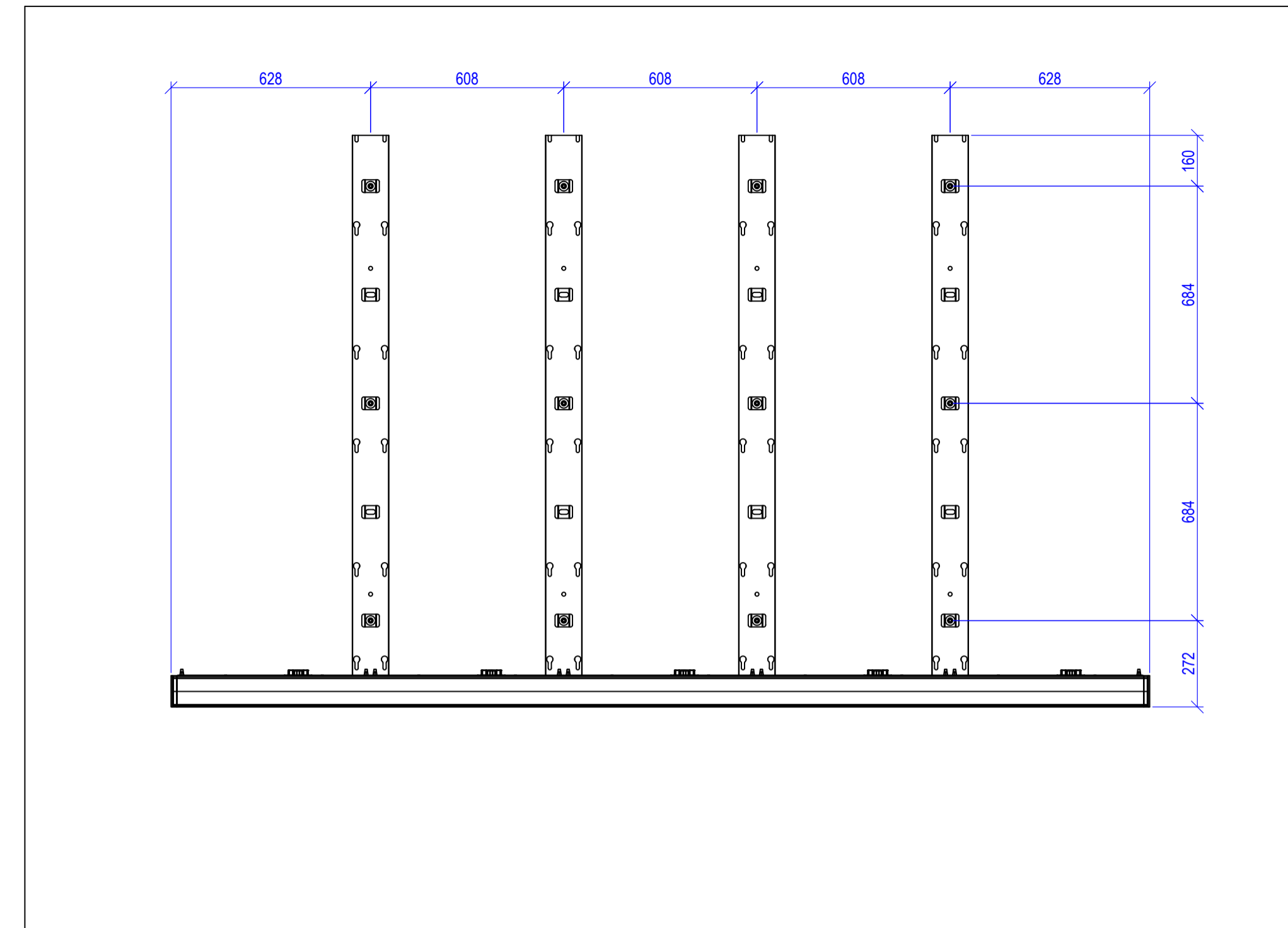
Front View Structure
