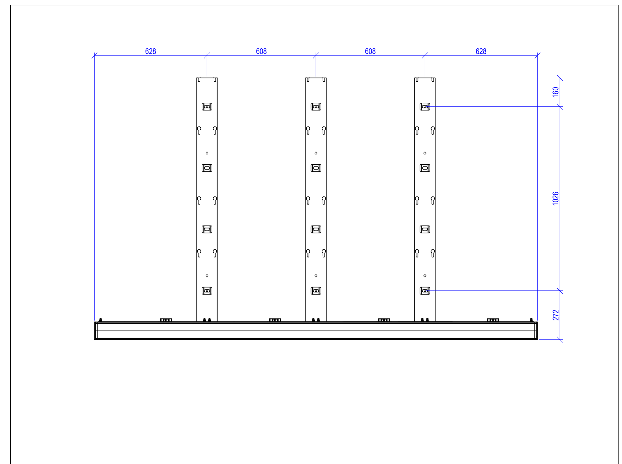
Front View Structure
