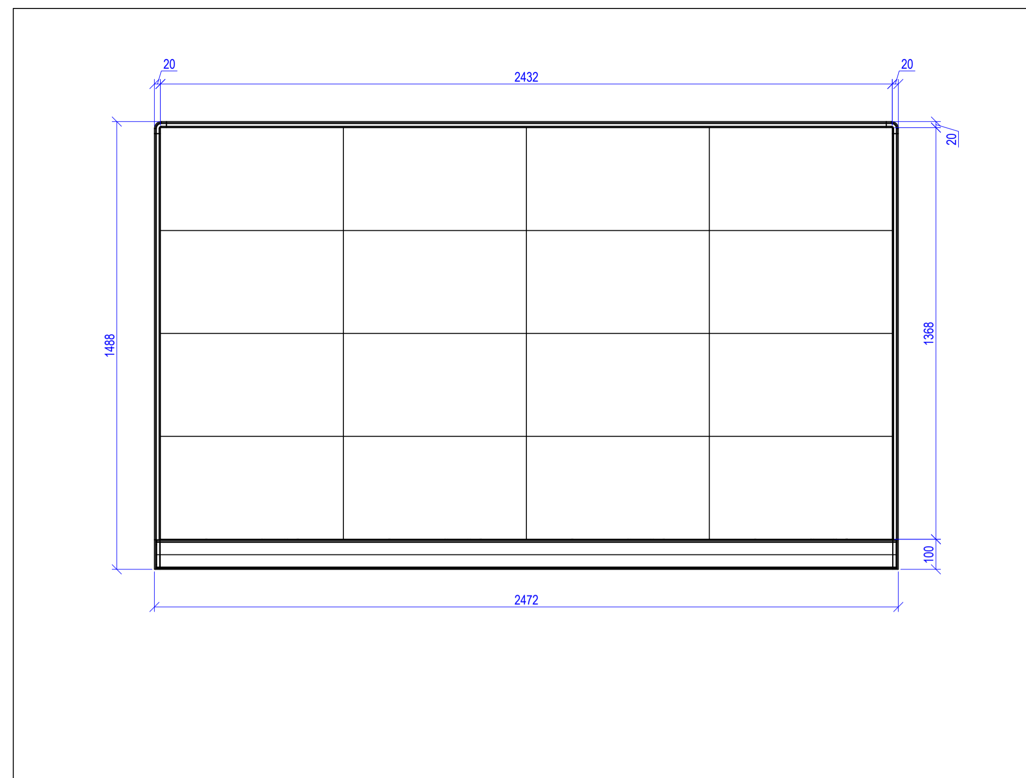
Front View
