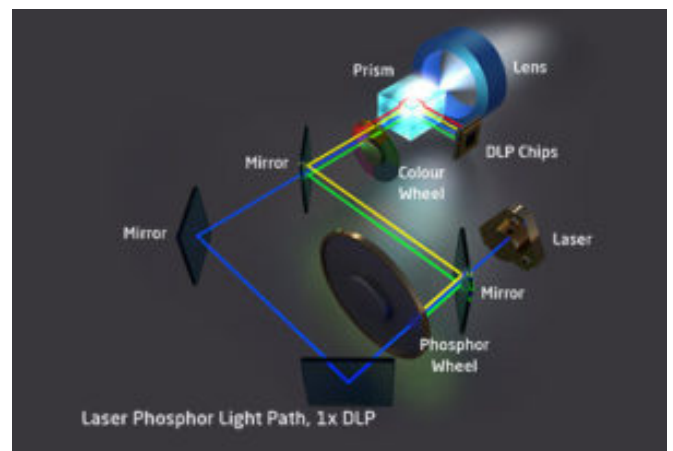
NEC provided image of their laser light engine design.
